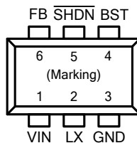
Figure 1. Pin Assignments of FR9206
