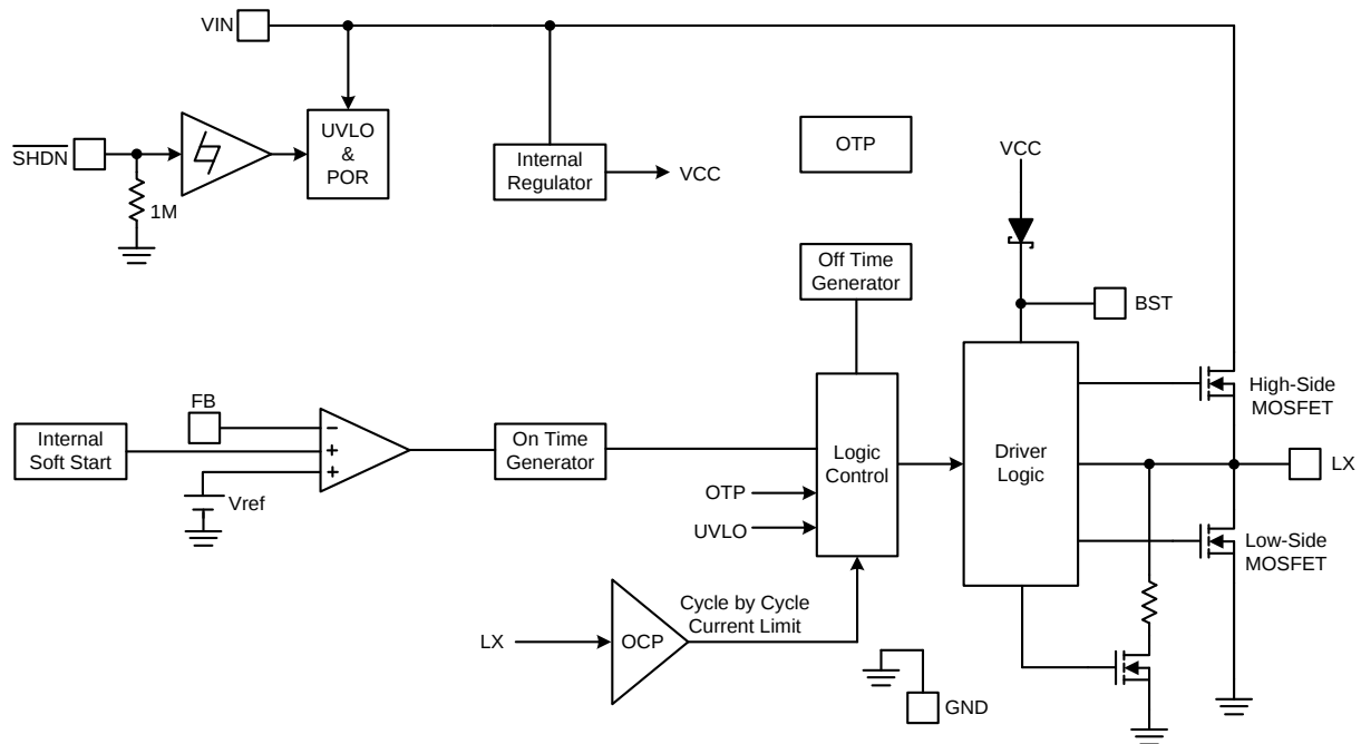
Figure 4. Block Diagram of FR9206
